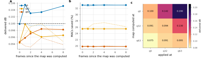
Figure 33. Reusing an exit map. Solid is the transferred map, dashed the one recomputed in place. a , b : reuse across frames of the same sequence. c : reuse across quality index; the entry is the delivered distortion against a 0.1 dB budget.
