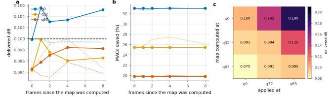
Figure 33. Reusing an exit map. Solid is the transferred map, dashed the one recomputed in place. a, b: reuse across frames of the same sequence. c: reuse across quality index; the entry is the delivered distortion against a 0.1 dB budget.
