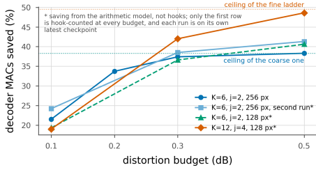
Figure 34. The right ladder depends on the budget. Saving against budget for four ladders, with each one’s architectural ceiling as a dotted line. A finer ladder has a higher ceiling and a higher floor, so the curves cross: the coarse ladder wins where the budget is tight and cannot be spent, and the fine one wins where it is loose enough to reach exits the coarse ladder does not have. The crossing is the design choice this section is about.
