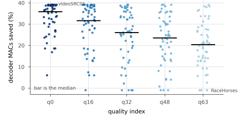
Figure 20. What the set mean hides. Every test sequence as a point, at the 0.1 dB budget; the bar is the median. At the lowest rate the saving runs from 6.0% to 39.1% across the 53 sequences and at the highest from -1.0% to 39.1%. The spread within a rate is larger than the difference between rates, and it is content, not noise: the same sequences sit at the same end of it at every rate.
