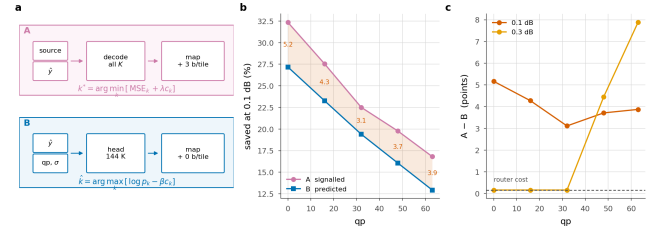
Figure 27. Who decides. a , the two decision paths side by side: the encoder's search over all K exits per tile against the head's forward pass over decoded data. b , saving at 0.1 dB; shading is what a bit-exact bitstream costs. c , that cost is smallest at q32 and grows in both directions.
