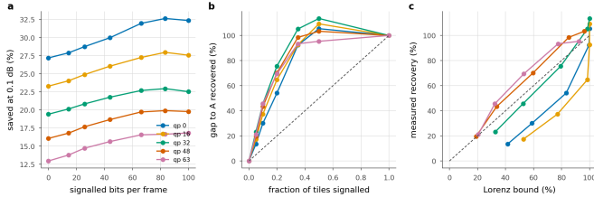
Figure 31. Partial signalling. a, saving against the bits spent on the map; each line runs from B on the left to A on the right. b, the same normalised by the A-to-B gap; dashed is proportional recovery. c, against the fixed- \lambda Lorenz bound; points above the dashed line are allocations one multiplier cannot reach.
