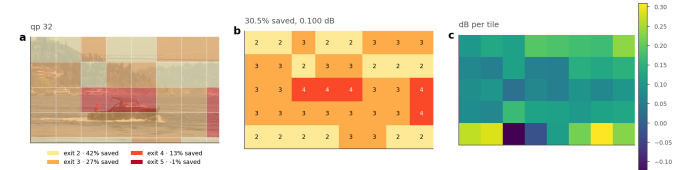
Figure 18. Where the decoder spends. Bosphorus at q32, a 0.1 dB budget. (a) the assignment overlaid on the frame, (b) the exit index per tile, (c) the quality each tile gives up, against its own full-depth reference. Water and sky leave at the shallowest exit; the boat and the shoreline run deep.
