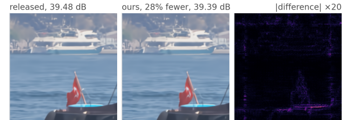
Figure 30. What 28.1% of the arithmetic costs, to look at. Bosphorus at q32, one frame, with \lambda bisected on that frame to 0.100 dB. Both crops are decoded from the same latent at 0.2743 bpp: the released decoder reaches 39.48 dB and the routed decode 39.39 dB. The crop is centred on the tile that gave up the most, tile 18 of 40, not on a flattering one. Right, the absolute difference at \times 20 .
