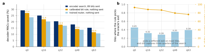
Figure 29. Three ways to choose an exit. a , saving at 0.1 dB. The encoder search sees the source and sends 89 bits a frame; the other two send nothing. The bit rule beats the trained head at every rate, with no learned parameters against the head's 144,030. b , bars are the tiles where the rule picks the search's exit, the line the fraction of its saving it captures anyway.
