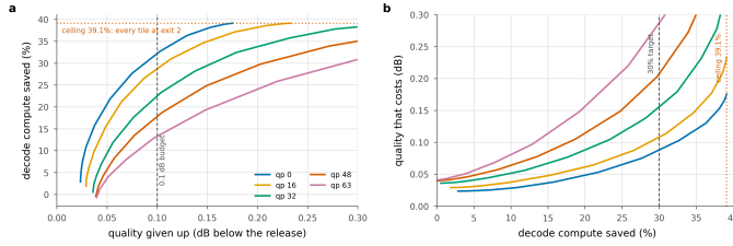
Figure 25. The trade-off, whole. a What a budget buys, per rate; the dotted line is the arithmetic ceiling, 39.1%, and q_0 reaches it at 0.179 dB. b The same relation inverted, so it reads as what a saving target costs. The three budgets reported elsewhere are three points on this curve.
