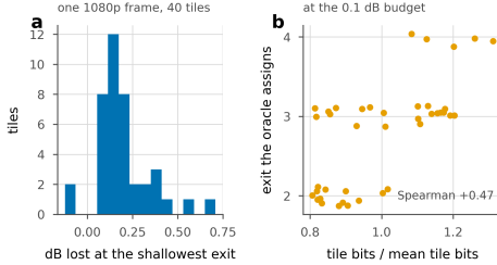
Figure 2. Why depth should not be uniform. One 1080p frame, 40 tiles. a , what each tile loses at the shallowest exit the ladder allows: a few lose nothing measurable and one loses 0.71 dB, and a single depth has to be set by the worst of them. b , the bits already spent on a tile against the exit the oracle sends it to, at 0.1 dB.
