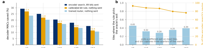
Figure 30. Three ways to choose an exit. a , saving at 0.1 dB. The encoder search sees the source and sends 89 bits a frame; the other two send nothing. The bit rule beats the trained head at every rate, with no learned parameters against the head's 144,030. b , bars are the tiles where the rule picks the search's exit, the line the fraction of its saving it captures anyway.
