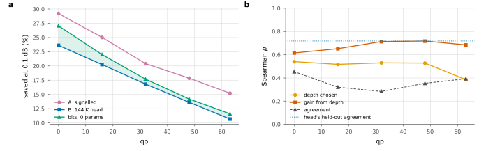
Figure 28. The calibrated bit rule. a Saving at 0.1 dB; shaded where the calibrated bit rule beats the trained head. b What a tile's bit count is correlated with, against how often the rule agrees with the oracle outright; dotted is the head's own held-out agreement.
