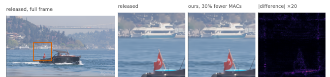
Figure 7. What the saving looks like. The same bitstream decoded by the released decoder and by ours at the 0.1 dB operating point, 30.5% fewer
