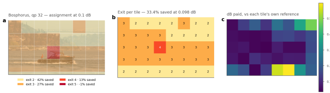
Figure 9. Where the decoder spends. (a) the assignment overlaid on the frame, (b) the exit index per tile, (c) the quality each tile gives up against its own full-depth reference. Water and sky leave at the shallowest rung; the boat and shoreline run deep.
