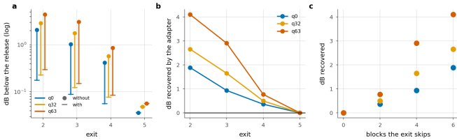
Figure 4. What the adapters are worth. a, each exit with and without its adapter. b, the dB the adapter recovers. c, the same against the number of blocks the exit skips — the design rationale, measured.
