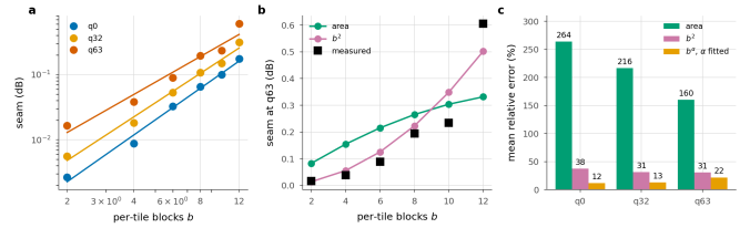
Figure 6. The seam against per-tile depth. Sweeping the split depth sweeps b ; b=0 is an exact control and measures 0.0000 dB at all three rates. a , the measurement with the fitted power law. b , both models against q_{63} with one free scale each. c , mean relative error. The area fraction saturates once every pixel is contaminated; the penalty does not.
