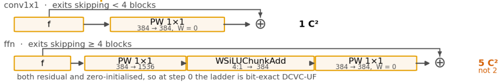
Figure 3. Inside the boxes of Figure 1. a Tiling is a reshape and nothing else — no arithmetic, and no information crosses a tile border afterwards, which is the whole cost and the whole benefit. b One exit group is two DepthConvBlocks; the single 3×3 depthwise is the only operator with spatial extent, hence the only source of the seam, at 0.29% of the block. c Both adapters are pointwise, residual and zero-initialised, so the ladder starts as the released decoder exactly. The FFN adapter costs 5C 2 , which the cost model billed as 2C 2 until it was measured against the module.
