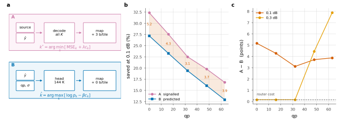
Figure 17. Who decides. (a) A holds the source, so it can decode all K exits per tile and pick the true minimiser; it signals the map at \sim 90 bits/frame. B never sees the source — a 144 K-parameter head reads y -hat, the entropy scales and qp — and signals nothing. (b) Saving at 0.1 dB; shading is what a bit-exact bitstream costs. (c) That cost is smallest at q32, where the tilt needed to move the router off its training multiplier is essentially zero, and grows in both directions. At 0.3 dB it collapses to the router's own 0.163% wherever the budget saturates the ladder, and widens where it does not.
