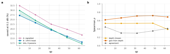
Figure 18. The free baseline. a Saving at 0.1 dB; shaded where the parameter-free rule beats the trained head. b What a tile's bit count is correlated with, against how often the rule agrees with the oracle outright; dotted is the head's own held-out agreement.
