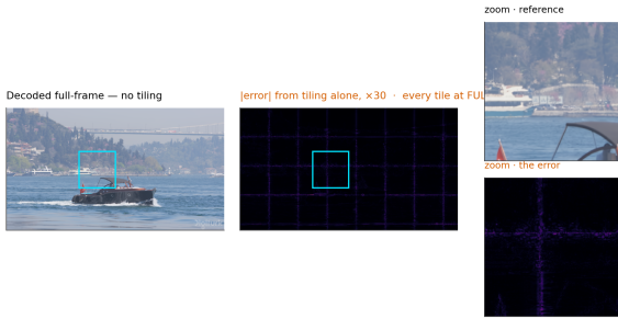
Figure 5. The artefact, before anything is done about it. One frame decoded twice from the same bitstream with the same weights, every tile at full depth, stock zero padding — no early exit anywhere. The only difference is that the right-hand decode was tiled. The error map is the tile lattice and nothing else.
