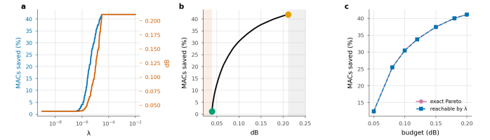
Figure 14. The structure of the allocation, on one frame. a , compute and distortion are monotone in the multiplier. b , the frontier between the floor (green) and saturation (orange); shaded regions are infeasible and wasted. c , what the Lagrangian reaches against the exact Pareto set, enumerated by dynamic programming — the two curves are indistinguishable.
