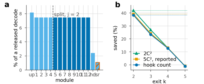
Figure 40. Where the arithmetic is, and what an exit saves. a , one released decode by module: the opening upsample, the twelve trunk blocks, the head, and the seam-repair pass this work adds (hatched). Light bars always run; dark bars are the eight blocks after the split that a tile can skip. b , the saving at each reachable exit under three prices for the same architecture, with each price's ceiling dotted. Section B.5 is the table behind it.
