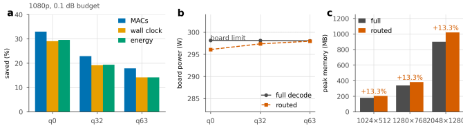
Figure 35. Three units for one saving. a , the same routed decode measured as arithmetic, as wall clock and as joules per frame, at 1080p and a 0.1 dB budget. Energy follows the clock, not the arithmetic. b , why: the board draws the same power either way, because the later groups run on a shrinking set of tiles and a partly idle GPU still draws its static power. c , peak memory, which routing raises rather than lowers, by 13.3% at every resolution that fitted on the card.
