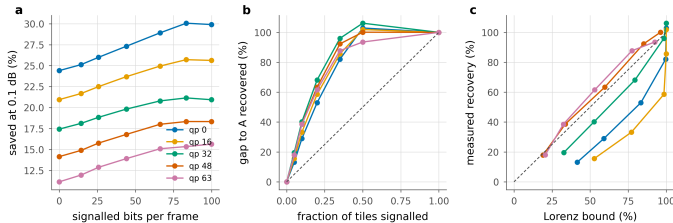
Figure 32. Partial signalling. a, saving against the bits spent on the map; each line runs from B on the left to A on the right. b, the same normalised by the A-to-B gap; dashed is proportional recovery. c, against the fixed- \lambda Lorenz bound; points above the dashed line are allocations one multiplier cannot reach.
