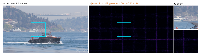
Figure 61. The seam, at frame scale. a, the decoded frame. b, the absolute error against a full-frame decode of the same latent, amplified 30x, with every tile at the deepest exit so that nothing here is early exiting. c, a zoom on one junction. The tile grid is the error: 0.124 dB at q63, paid before the allocation begins.
