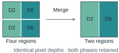
a Same map, fewer independent regions Neural decoder MACs: -12.44% (not latency)
