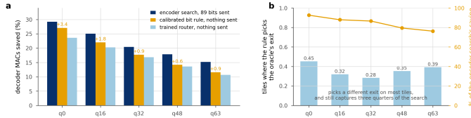
Figure 30. Three ways to choose an exit. a, saving at 0.1 dB. The encoder search sees the source and sends 89 bits a frame; the other two send nothing. The bit rule beats the trained head at every rate, with no learned parameters against the head's 144,030. b, bars are the tiles where the rule picks the search's exit, the line the fraction of its saving it captures anyway.
