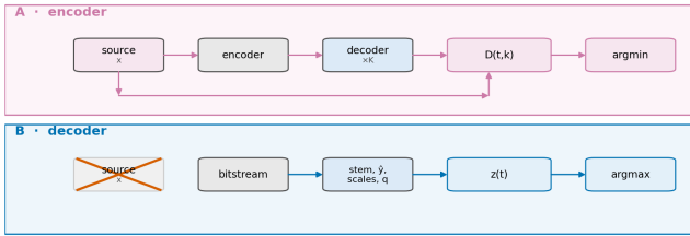
Figure 5. What each side knows. Configuration A, above, has the source frame, so it can decode a tile at every exit and measure D(t, k) directly; the map it finds then has to be carried in the bitstream. Configuration B, below, has no source frame. It sees the bitstream and whatever the decode has produced by the time the trunk splits, and turns that into one score vector z(t) per tile.
