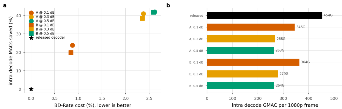
Figure 3. The same measurement drawn. Left, BD-Rate cost against compute saved, with the released decoder at the origin: the two configurations sit almost on top of each other in BD-Rate, and loosening the budget moves both up and to the right together. Right, decode cost per 1080p frame in GMAC. Rendered from the same run as the previous table, so the compute axis carries the same superseded cost model and the BD-Rate axis does not.
