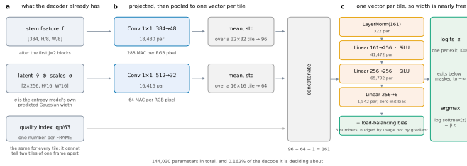
Figure N. The router head. a , the three things it reads, all already held by the decoder. b , each projected by a 1 \times 1 , then reduced to one vector per tile by its mean and standard deviation. c , a three-layer perceptron, one pass per tile. Every shape and parameter count is read off the module when the figure is drawn.
