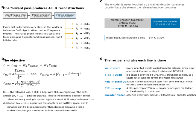
Figure 1. The training scheme. Panel (a): one forward pass produces all K reconstructions, so the ladder is trained as one object. Panel (b): the three loss terms. Panel (c): the encoder is never touched. Panel (d): why each line of the recipe is there. The figure is a schematic drawn from the model definition; the numbers it carries are parameter counts, and no file in results/ records those, which is why they are not quoted in the text.
