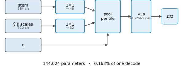
Figure 6. The head. Two 1 \times 1 projections, pooling to one vector per tile, then a perceptron. The parameter count and the compute share drawn on the figure are the measured ones from results/router_latency.json.
