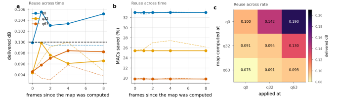
Figure 15. Reusing an exit map. Solid is the transferred map, dashed the one recomputed in place. a, b : reuse across frames of the same sequence. c : reuse across quality index; the entry is the delivered distortion against a 0.1 dB budget.
