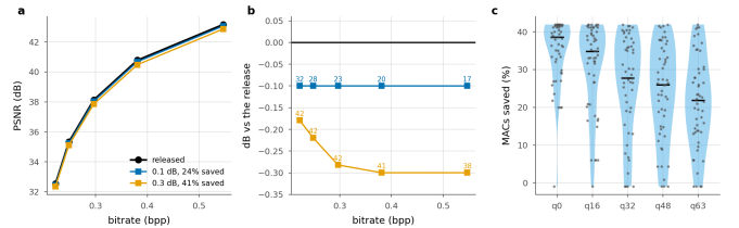
Figure 16. The plane a codec is read on, and the spread behind the mean. a, operating points against the released curve. b, the same with the quality axis expanded; labels are compute saved. c, per sequence at a matched point near 0.1 dB; one dot per sequence, bar is the median.
