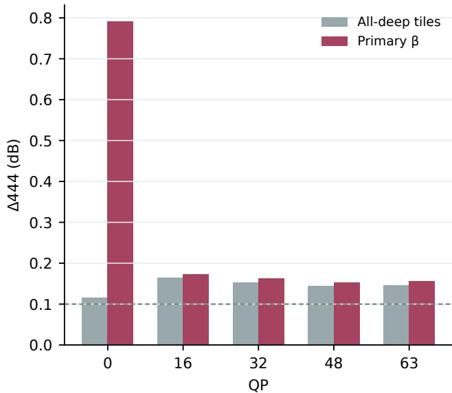
b No scalar \beta meets 0.10 dB: image 0828
