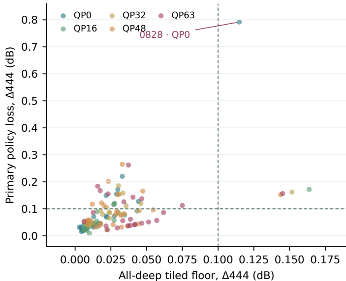
a Scalar price cannot remove the tile floor
