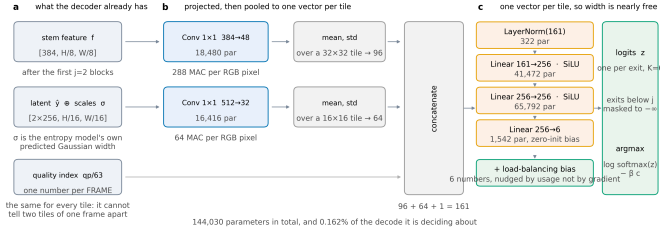
Figure 60. The router head. a , the three things it reads, all already held by the decoder at the moment the decision is needed. b , each projected by a 1×1, then reduced to one vector per tile by its mean and standard deviation. c , a three-layer perceptron, one pass per tile. Every shape and parameter count in the figure is read off the module when the figure is drawn.
