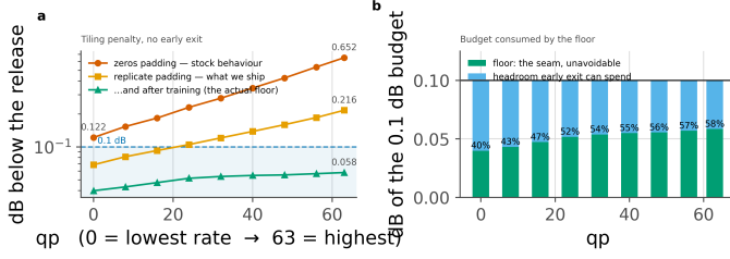
Figure 55. The tiling penalty across the whole rate range , every tile at full depth, so this is the floor and nothing else. a , the steps that reduce it, of which the two that matter cost no arithmetic; the largest single factor is training the ladder with the seam present. b , the floor as a share of the 0.1 dB budget: it is charged inside the budget and consumes a growing part of it as the rate rises, which is one of the two reasons the saving falls with rate.
