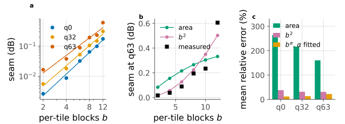
Figure 12. The seam against per-tile depth. a , the measurement with the fitted power law. b , both models against q63, one free scale each. c , mean relative error. The area fraction saturates once the border reaches every pixel; the penalty does not.
