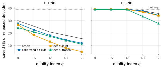
Figure 56. The rule sits between the two heads and the oracle. Saving at each rate, against the Lagrangian oracle measured inside the same run and the architectural ceiling (dotted). At 0.1 dB the rule is above both heads at every rate, and the gap between the two heads is wider than the gap between the rule and either of them. At 0.3 dB the three lowest rates saturate and the three curves separate only at q48 and q63.
