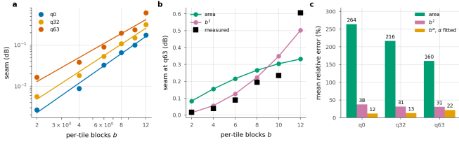
Figure 60. The seam against per-tile depth. a , the measurement with the fitted power law. b , both models against q63, one free scale each. c , mean relative error. The area fraction saturates once the border reaches every pixel and the penalty does not, which is where the area law fails as a predictor.
