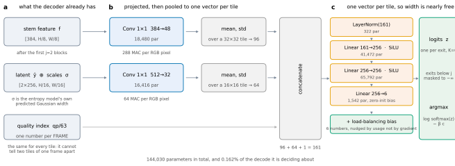
Figure 55. The router head. a , the three things it reads, all already held by the decoder at the moment the decision is needed. b , each projected by a 1 \times 1 , then reduced to one vector per tile by its mean and standard deviation. c , a three-layer perceptron, one pass per tile. Every shape and parameter count in the figure is read off the module when the figure is drawn.
