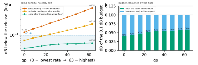
Figure 50. The tiling penalty across the whole rate range, every tile at full depth, so this is the floor and nothing else. a, the steps that reduce it, of which the two that matter cost no arithmetic; the largest single factor is training the ladder with the seam present. b, the floor as a share of the 0.1 dB budget: it is charged inside the budget and consumes a growing part of it as the rate rises, which is one of the two reasons the saving falls with rate.
