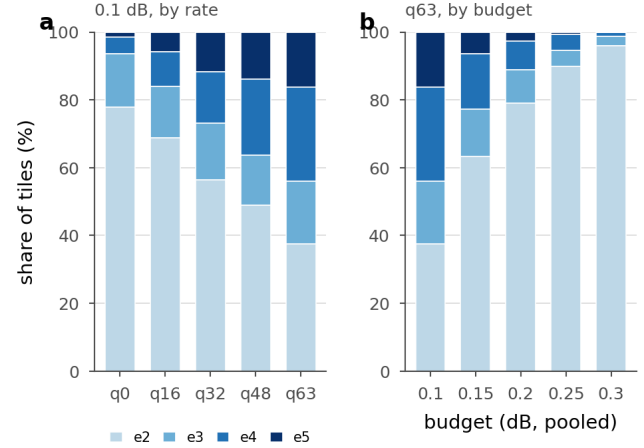
Figure 44. How the ladder fills up. a , exit shares at the 0.1 dB budget as the rate rises. b , exit shares at q63 as the budget loosens, until at 0.3 dB 96% of tiles are already at the shallowest exit and there is almost nothing left to allocate. Both panels are pooled over the test set.
