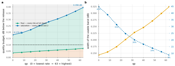
Figure 49. Three regions, and only the middle one is a design choice. Below the floor no allocation meets the budget; above saturation every tile already takes the cheapest exit and a looser budget buys nothing. The 0.1 dB budget uses 45% of the band at the lowest rate and 9% at the highest, which is why the same budget behaves so differently at the two ends of the rate range.
