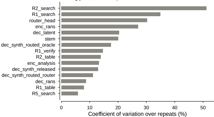
Timing jitter, one 1080p frame \times 10
