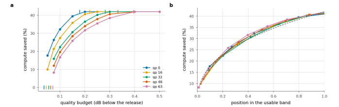
Figure 21. The band is the rate dependence. a Saving against the budget, with each rate's floor and saturation point ticked. b The same with the budget axis rescaled onto each rate's own band. Five curves become one; dashed is the one-parameter power law fitted to all of them.
