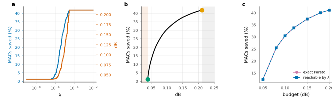
Figure 20. The structure of the allocation, on one frame. a, compute and distortion are monotone in the multiplier. b, the frontier between floor and saturation; shaded regions are infeasible or wasted. c, what the Lagrangian reaches against the exact Pareto set, enumerated by dynamic programming.
