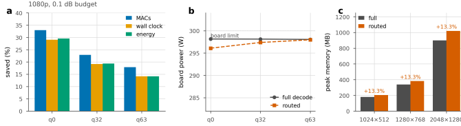
Figure 30. Three units for one saving. a, the same routed decode measured as arithmetic, as wall clock and as joules per frame, at 1080p and a 0.1 dB budget. Energy follows the clock, not the arithmetic. b, why: the board draws the same power either way, because the later groups run on a shrinking set of tiles and a partly idle GPU still draws its static power. c, peak memory, which routing raises rather than lowers, by 13.3% at every resolution that fitted on the card.
