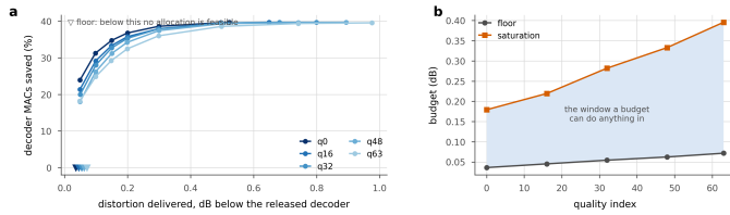
Figure 23. The window a budget works in. a , saving against the distortion actually delivered, per rate. Every curve begins at a floor, below which no allocation meets the budget, and flattens at a saturation point, above which a looser budget buys nothing. b , those two limits against rate. The shaded band is the only region in which a budget is a design choice rather than a formality.
