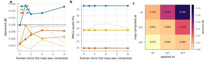
Figure 29. Reusing an exit map. Solid is the transferred map, dashed the one recomputed in place. a , b : reuse across frames of the same sequence. c : reuse across quality index; the entry is the delivered distortion against a 0.1 dB budget.
