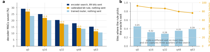
Figure 26. Three ways to choose an exit. a , saving at the 0.1 dB budget. The encoder search sees the source and sends 89 bits a frame; the other two send nothing. The bit rule beats the trained head at every rate, by the margin printed above it, with no learned parameters against the head's 144,030. b , bars are the tiles on which the rule picks the exit the search would have, and the line is the fraction of the search's saving it nonetheless captures. Picking a different exit on most tiles costs it far less than picking a different exit sounds like it should, which is the case against training a router on exit labels.
