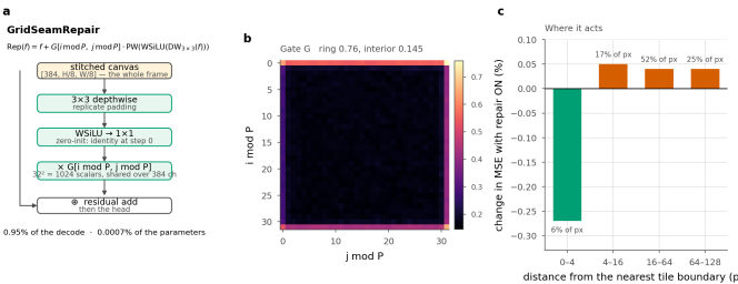
Figure 6. Grid seam repair. A correction gated by position within a tile, applied once to the stitched frame. The trained gate learns the boundary ring (0.76) but never switches off inside (0.145 over 94% of pixels), and the measured effect follows: it helps on the ring and hurts everywhere else.
