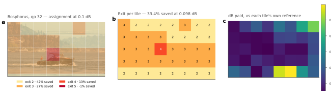
Figure 9. Where the decoder spends. (a) the assignment overlaid on the frame, (b) the exit index per tile, (c) the quality each tile gives up against its own full-depth
