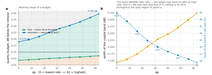
Figure 11. Three regions, and only the middle one is a design choice. Below the floor no allocation meets the budget; above saturation every tile is already on the cheapest rung. The working 0.1 dB budget uses 45% of the window at the lowest rate and 9% at the highest.
