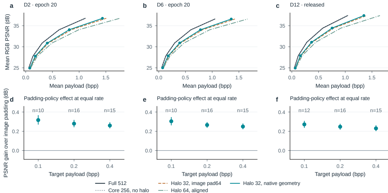
Figure S23. Keep spatial rounding inside the codec contract. a–c. Actual-payload RD points averaged over the fixed 16-image cohort, with shared axis limits. d–f. Per-image matched-rate gain from moving padding to the latent, with paired 95% image-bootstrap intervals. Each rate uses the common support of all five variants within that depth; n denotes supported images out of 16, with no extrapolation. The latent-padding implementation uses CPU FP32 research streams; “native geometry” does not denote native CUDA output or latency.
