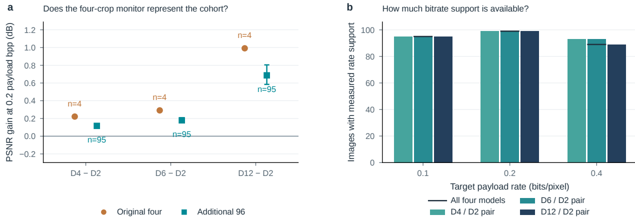
Figure S11. Coverage is part of the result. a , Original monitor crops and additional images at 0.2 payload bpp, restricted to four-model common support. We do not estimate uncertainty from the four-crop subset. b , Pairwise and four-model supported counts at each target rate. A changing cohort is made explicit rather than filled by extrapolation.
