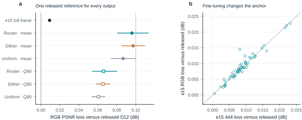
Figure S18. Measure the anchor before interpreting the loss budget. The same 53 first frames, QP32, valid-pixel support and CPU FP32 reconstruction. a , e15 full-frame and six fixed policies relative to released D12; points and intervals show means and paired 95% sequence-bootstrap intervals. Filled circles use mean control and hollow squares Q90; the dark full-frame point measures anchor drift. The dashed 0.1 dB line is a numerical reference. b , Per-sequence e15 drift under equal-channel unclipped 444 and converted/clipped RGB. The diagonal denotes metric agreement. No output or policy is reselected when the reference changes.
