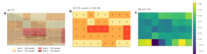
Figure 18. Where the decoder spends. Bosphorus at q32, a 0.1 dB budget. (a) the assignment overlaid on the frame, (b) the exit index per tile, (c) the quality each tile gives up, against its own full-depth reference. Water and sky leave at the shallowest exit; the boat and the shoreline run deep.
