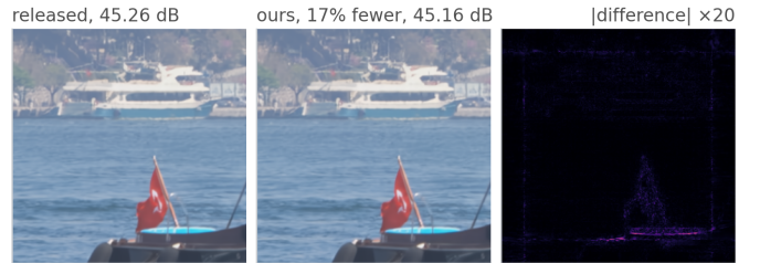
Figure 36. The same frame at the top of the rate range. Bosphorus at q63, 0.4653 bpp, the same 0.1 dB budget and the same crop as Figure 30. The released decoder reaches 45.26 dB and the routed decode 45.16 dB, for 17.4% of the arithmetic rather than 28.1%.
