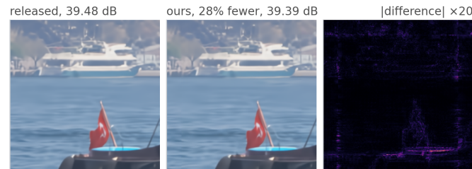
Figure 30. What 28.1% of the arithmetic costs, to look at. Bosphorus at q32, one frame, with \lambda bisected on that frame to 0.100 dB. Both crops are decoded from the same latent at 0.2743 bpp: the released decoder reaches 39.48 dB and the routed decode 39.39 dB. The crop is centred on the tile that gave up the most, tile 18 of 40, not on a flattering one. Right, the absolute difference at \times 20 .
