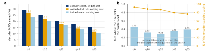
Figure 29. Three ways to choose an exit. a , saving at 0.1 dB. The encoder search sees the source and sends 89 bits a frame; the other two send nothing. The bit rule beats the trained head at every rate, with no learned parameters against the head's 144,030. b , bars are the tiles where the rule picks the search's exit, the line the fraction of its saving it captures anyway.
