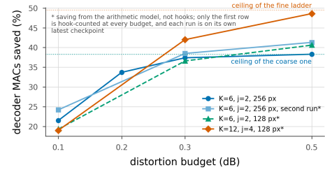
Figure 34. The right ladder depends on the budget. Saving against budget for four ladders, with each one's architectural ceiling as a dotted line. A finer ladder has a higher ceiling and a higher floor, so the curves cross: the coarse ladder wins where the budget is tight and cannot be spent, and the fine one wins where it is loose enough to reach exits the coarse ladder does not have. The crossing is the design choice this section is about.
