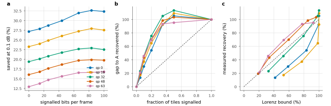
Figure 31. Partial signalling. a, saving against the bits spent on the map; each line runs from B on the left to A on the right. b, the same normalised by the A-to-B gap; dashed is proportional recovery. c, against the fixed- \lambda Lorenz bound; points above the dashed line are allocations one multiplier cannot reach.
