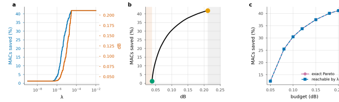
Figure 23. The structure of the allocation, on one frame. a , compute and distortion are monotone in the multiplier. b , the frontier between floor and saturation; shaded regions are infeasible or wasted. c , what the Lagrangian reaches against the exact Pareto set, enumerated by dynamic programming.
