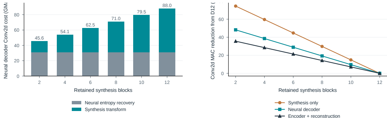
Figure S8. The arithmetic denominator changes the apparent saving. a , Synthesis varies with depth while neural entropy recovery stays fixed. b , The same architectural intervention under three accounting scopes. Counts use 512 \times 512 input and one MAC per multiply-accumulate; they are not observed kernel times. D8/D10 are architecture-only controls. Encoder totals include reconstruction but omit rANS, elementwise work, transfers and control overhead.
