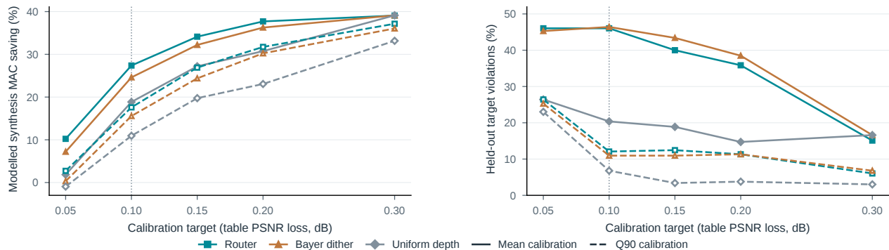
Figure S5. A source-free control trades arithmetic savings against tail risk. Controls are calibrated on other sequences, separately at each QP, using the training mean (solid) or 90th percentile (dashed). All 265 pairs are retained, including cases from infeasible calibration groups. a , Modelled MAC saving. b , Fraction exceeding the table-loss target. These padded source-error diagnostics do not establish final mixed-image quality, a per-frame guarantee or complete decoder speed.
