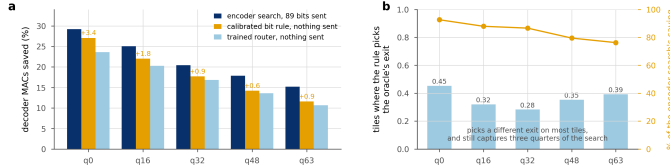
Figure 29. Three ways to choose an exit. a , saving at 0.1 dB. The encoder search sees the source and sends 89 bits a frame; the other two send nothing. The bit rule beats the trained head at every rate, with no learned parameters against the head's 144,030. b , bars are the tiles where the rule picks the search's exit, the line the fraction of its saving it captures anyway.
