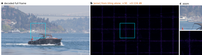
Figure 63. The seam, at frame scale. a , the decoded frame. b , the absolute error against a full-frame decode of the same latent, amplified 30 \times , with every tile at the deepest exit so that nothing here is early exiting. c , a zoom on one junction. The tile grid is the error: 0.124 dB at q63, paid before the allocation begins.
