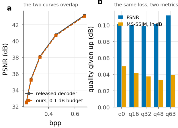
Figure 45. a , the rate-quality curve of the released decoder and of ours at the 0.1 dB budget, over the five quality indices. At plot scale they are one curve, which is what a 0.1 dB budget means. b , the gap that panel a cannot show, in PSNR and in MS-SSIM expressed as a decibel.
