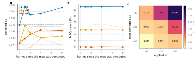
Figure 33. Reusing an exit map. Solid is the transferred map, dashed the one recomputed in place. a, b: reuse across frames of the same sequence. c: reuse across quality index; the entry is the delivered distortion against a 0.1 dB budget.
