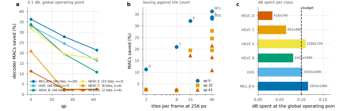
Figure 12. Saving by test class at one global operating point. \lambda is bisected once so the whole set lands on the budget, exactly as it would be in deployment; each class is then reported at that \lambda . The ordering follows tile count, not content.
