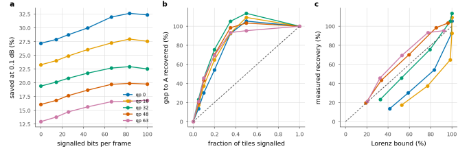
Figure 19. Partial signalling. a , saving against the bits spent on the map; each line runs from B on the left to A on the right. b , the same normalised by the A-to-B gap; dashed is proportional recovery. c , against the fixed- \lambda Lorenz bound; points above the dashed line are allocations one multiplier cannot reach.
