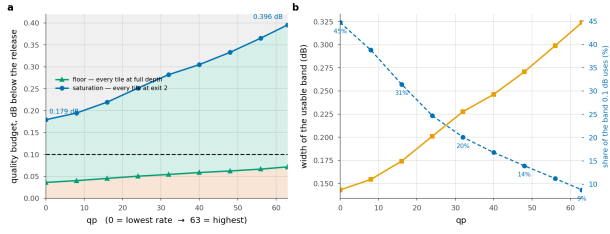
Figure 13. Three regions, and only the middle one is a design choice. Below the floor no allocation meets the budget; above saturation every tile already takes the cheapest exit. The 0.1 dB budget uses 45% of the band at the lowest rate and 9% at the highest.
