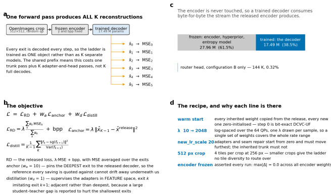
Figure 26. The training scheme. Panel (a): one forward pass produces all K reconstructions, so the ladder is trained as one object. Panel (b): the three loss terms. Panel (c): the encoder is never touched. Panel (d): why each line of the recipe is there. The figure is a schematic drawn from the model definition; the numbers it carries are parameter texts, and no file in results/ records those, which is why they are not quoted in the text.
