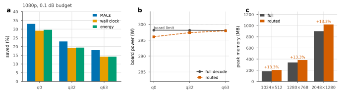
Figure 28. Three units for one saving. a , the same routed decode measured as arithmetic, as wall clock and as joules per frame. b , why they differ: the board draws the same power either way, because the later groups run on a shrinking set of tiles and a partly idle GPU still draws its static power. c , peak memory, which routing raises rather than lowers.
