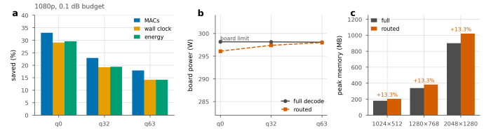
Figure 35. Three units for one saving. a , the same routed decode measured as arithmetic, as wall clock and as joules per frame, at 1080p and a 0.1 dB budget. Energy follows the clock, not the arithmetic. b , why: the board draws the same power either way, because the later groups run on a shrinking set of tiles and a partly idle GPU still draws its static power. c , peak memory, which routing raises rather than lowers, by 13.3% at every resolution that fitted on the card.
