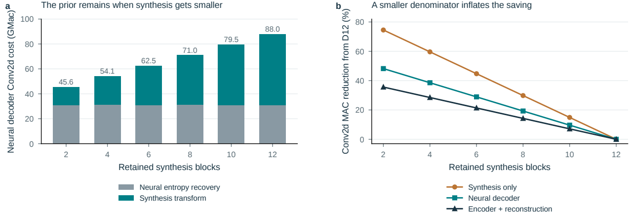
Figure S8. The arithmetic denominator changes the apparent saving. a , Synthesis varies with depth while neural entropy recovery stays fixed. b , The same architectural intervention under three accounting scopes. Counts use 512 \times 512 input and one MAC per multiply-accumulate; they are not observed kernel times. D8/D10 are architecture-only controls. Encoder totals include reconstruction but omit rANS, elementwise work, transfers and control overhead.
