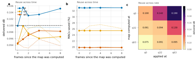
Figure 12. Reusing an exit map. Solid is the transferred map, dashed the one recomputed in place. a, b: reuse across frames of the same sequence. c: reuse across quality index; the entry is the delivered distortion against a 0.1 dB budget.
