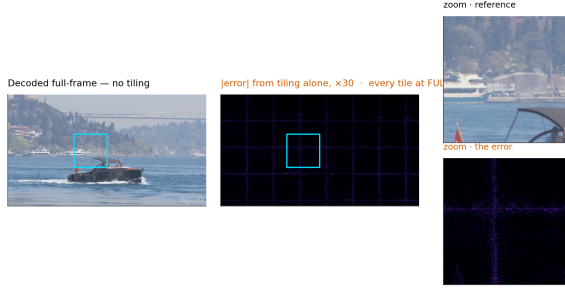
Figure 4. The artefact, before anything is done about it. One frame decoded twice from the same bitstream with the same weights, every tile at full depth — no early exit anywhere. The only difference is that the right-hand decode was tiled. The error map is the tile lattice and nothing else.
