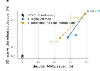
Figure 37. What the saving costs in rate. BD-rate against the released decoder, against the decoder MACs saved, for both configurations at the three budgets; each point is labelled with the budget that produced it. The star is the released decoder itself: no saving, no cost. Anchored on the same bitstream, so a BD-rate here is the price of decoding one file with fewer operations, not one codec against another.
