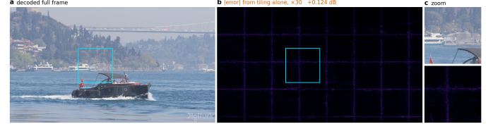
Figure 11. The artefact, before anything is done about it. Bosphorus at 1080p, quality index 63, zero padding at the tile border. a , the frame decoded in one piece. b , the same bitstream and weights decoded in 256 pixel tiles, every tile at full depth: the difference between the two, amplified 30 times. c , the boxed region of each.
