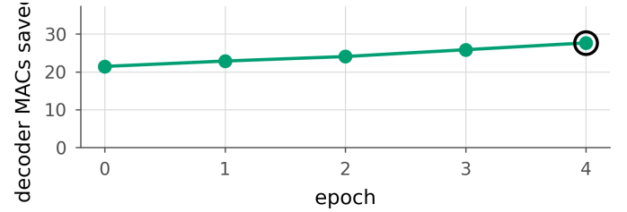
Figure 38. The run had not converged. Measured saving at the 0.1 dB budget on the 53 test frames, hook-counted, one point per completed epoch of the reported run. The circled point is the checkpoint this paper reports. The training loss over the same epochs is flat; the supplement shows the two together.
