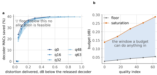
Figure 26. The window a budget works in. a, saving against the distortion actually delivered, per rate. Every curve begins at a floor, below which no allocation meets the budget, and flattens at a saturation point, above which a looser budget buys nothing. b, those two limits against rate. The shaded band is the only region in which a budget is a design choice rather than a formality.
