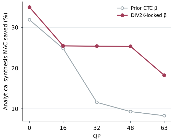
b Rate dependence on Kodak
