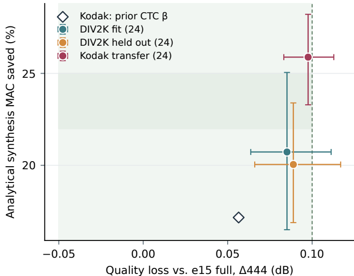
a Locked policy transfer
