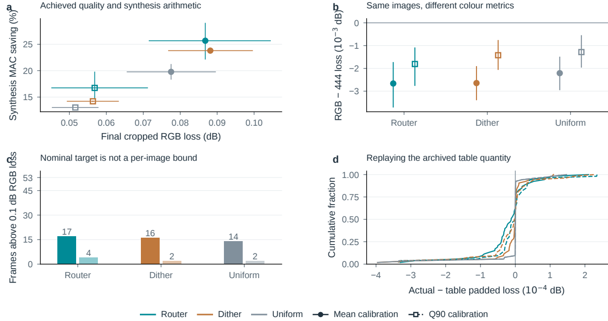
Figure S24. Carry the fixed decision through to the actual image. All 53 sequences at QP32, with no outcome-based exclusions. a , Achieved RGB loss and synthesis MAC saving with conditional 95% sequence-bootstrap intervals; these points are not an equal-quality frontier. b , RGB-minus-444 loss on the same support and reference. c , Counts above the nominal numerical threshold; pale bars denote Q90 calibration. d , Actual-minus-table loss on padded support. Mean and Q90 controls use a different calibration reference and metric from the cropped RGB report. The paired router-dither saving intervals include zero under both controls.
