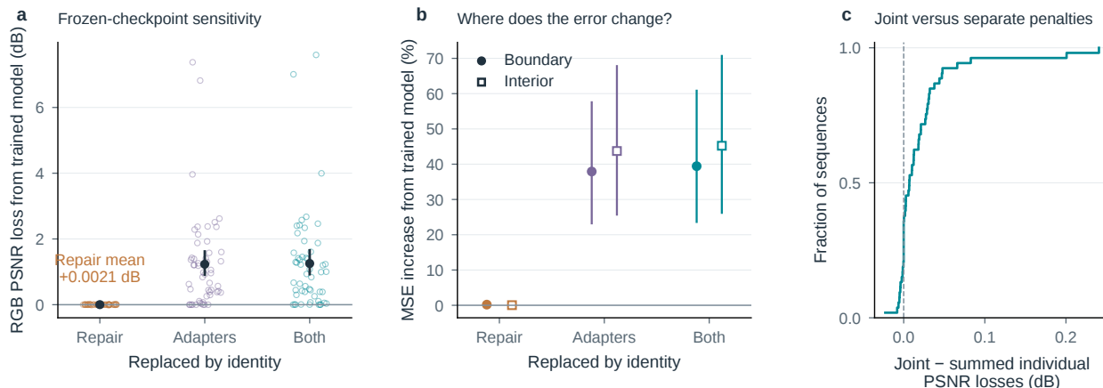
Figure S26. Separate learned dependence from architectural necessity. Fixed QP32, checkpoint and Q90 exit maps on all 53 first frames. a , RGB PSNR loss after identity substitution: individual sequences, means and paired 95% bootstrap intervals. b , Relative MSE change in boundary and interior pixels, averaged within sequence before aggregation. c , Joint-minus-summed individual PSNR penalties. This is a frozen-weight sensitivity test; it measures neither retrained alternatives nor runtime.
