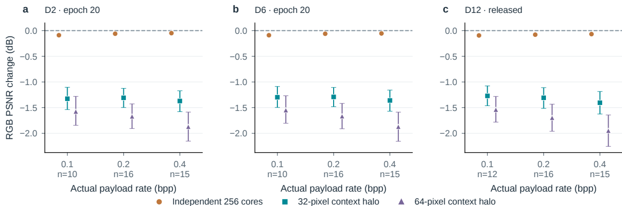
Figure S27. Charge repeated context to the transmitted rate. RGB PSNR changes from the same full-frame model at matched actual payload rate. Each depth uses the common supported images across full frame and all three patch variants; counts are shown and the vertical scale is shared. Intervals resample paired images. D2/D6 are interim epoch 20 models; D12 has different released training provenance. The experiment holds depth fixed within every contrast and makes no adaptive-routing or runtime claim.
