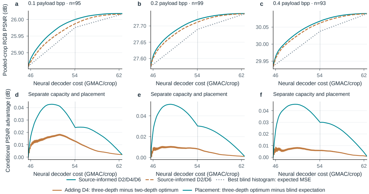
Figure S20. Separate the value of capacity choices from their assignment. Top: exact whole-crop allocation under a shared neural-decoder MAC budget. Bottom: incremental D4 option value and assignment premium over the best source-calibrated blind histogram’s expected MSE. Vertical guides mark the uniform-D4 budget. The curves use interpolated equal-rate quality and contain neither patch entropy resets nor a trained MLP. They are not within-image routing results or runtime frontiers.
