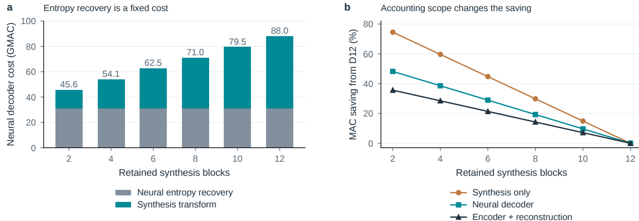
Figure S15. The arithmetic denominator changes the apparent saving. a , Synthesis varies with depth while neural entropy recovery stays fixed. b , The same architectural intervention under three accounting scopes. Counts use 512 \times 512 input and one MAC per multiply-accumulate; they are not observed kernel times. D8/D10 are architecture-only controls. Encoder totals include reconstruction but omit rANS, elementwise work, transfers and control overhead.
