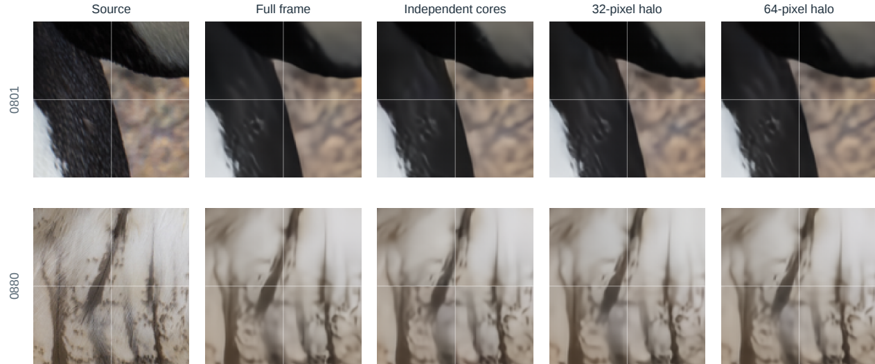
Figure S29. Predeclared views at the region intersection. D6 epoch 20, QP32, DIV2K 0801 and 0880. All panels use rows and columns 192:320 of the same 512-square crop; images and window were fixed before outcomes. The common light cross marks the patch boundary. Display images are rounded to 8 bit; numerical metrics use floating-point RGB. These are same-QP views, not equal-bitrate reconstructions.
