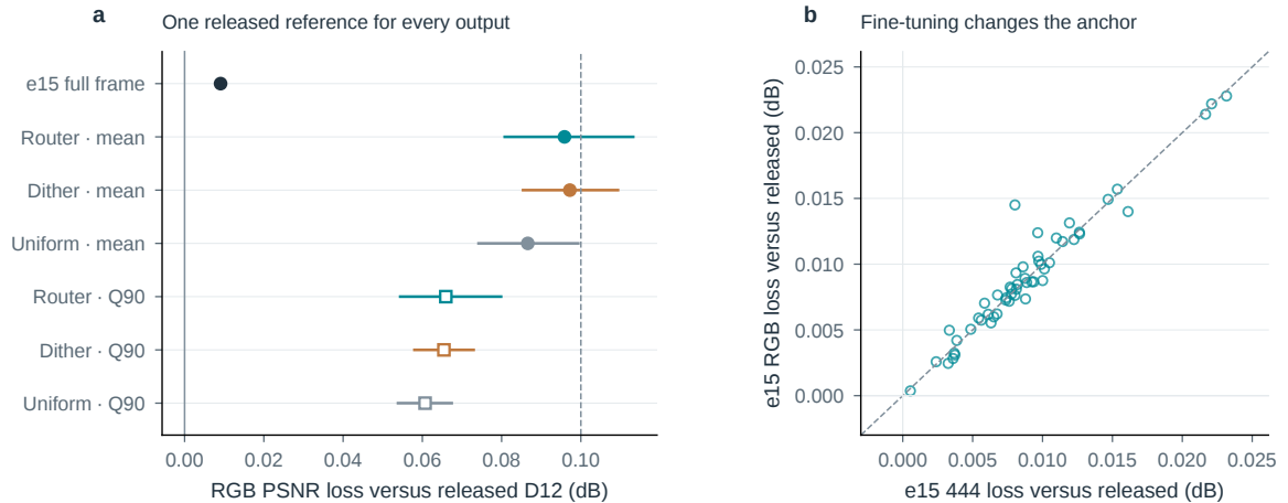
Figure S25. Measure the anchor before interpreting the loss budget. The same 53 first frames, QP32, valid-pixel support and CPU FP32 reconstruction. a , e15 full-frame and six fixed policies relative to released D12; points and intervals show means and paired 95% sequence-bootstrap intervals. Filled circles use mean control and hollow squares Q90; the dark full-frame point measures anchor drift. The dashed 0.1 dB line is a numerical reference. b , Per-sequence e15 drift under equal-channel unclipped 444 and converted/clipped RGB. The diagonal denotes metric agreement. No output or policy is reselected when the reference changes.
