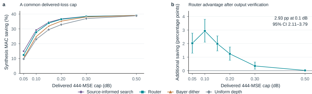
Figure S12. Controlling delivered loss within the recorded candidate pool. a , Maximum saving among actually measured eligible outputs, including a full-frame e15 fallback. b , Paired router–dither difference with 95% sequence-cluster intervals. All 265 pairs are retained, including explicit fallbacks, with YCbCr 4:4:4-loss tolerance 10^{-4} dB. This retrospective source-aware comparison excludes the cost of candidate generation and makes no released-reference or latency claim.
