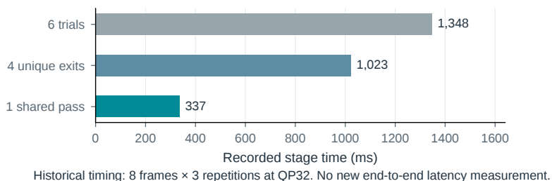
Figure S23. The decision path has an encoder cost. a , Stages required for source-error-based selection, with prefix reuse across candidate exits. b , Historical table-construction upper medians over 24 pooled trials, without invented uncertainty bars. c , A fixed held-out control and per-frame source calibration require different information. This is a stage analysis, not an end-to-end speedup.
