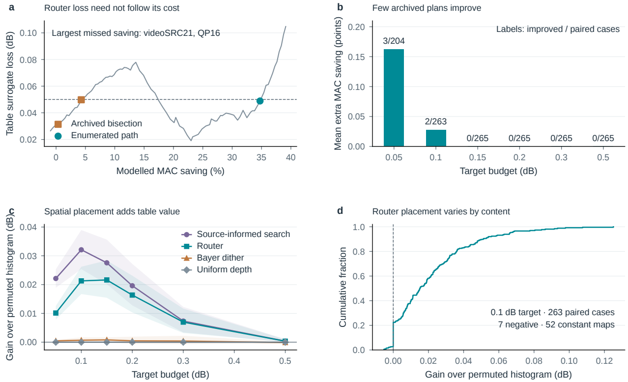
Figure S11. Control-path and assignment diagnostics. a , The explicitly selected largest missed router saving illustrates non-monotone table loss. b , Mean paired improvement from enumerating the router path; labels show improved and paired counts. Newly feasible cases are excluded from these means. c , Exact expected-shuffle comparison at unchanged exit histograms, with 95% sequence-cluster intervals. d , Router placement-gain distribution at 0.1 dB. All results are CPU analyses of padded error tables; none measures new final-image quality or latency.
