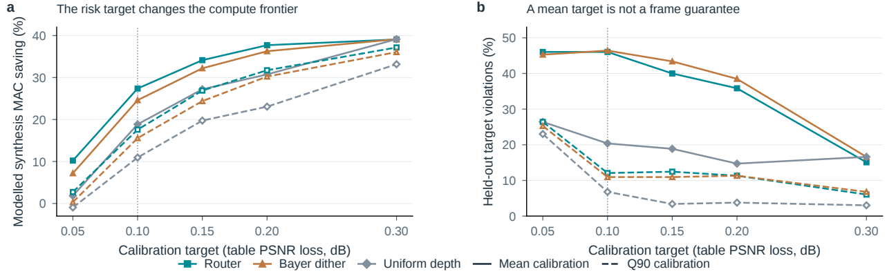
Figure S10. A source-free control trades arithmetic savings against tail risk. Controls are calibrated on other sequences, separately at each QP, using the training mean (solid) or 90th percentile (dashed). All 265 pairs are retained, including cases from infeasible calibration groups. a , Modelled MAC saving. b , Fraction exceeding the table-loss target. These padded source-error diagnostics do not establish final mixed-image quality, a per-frame guarantee or complete decoder speed.
