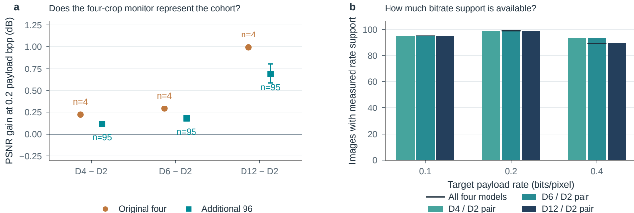
Figure S17. Coverage is part of the result. a , Original monitor crops and additional images at 0.2 payload bpp, restricted to four-model common support. We do not estimate uncertainty from the four-crop subset. b , Pairwise and four-model supported counts at each target rate. A changing cohort is made explicit rather than filled by extrapolation.
