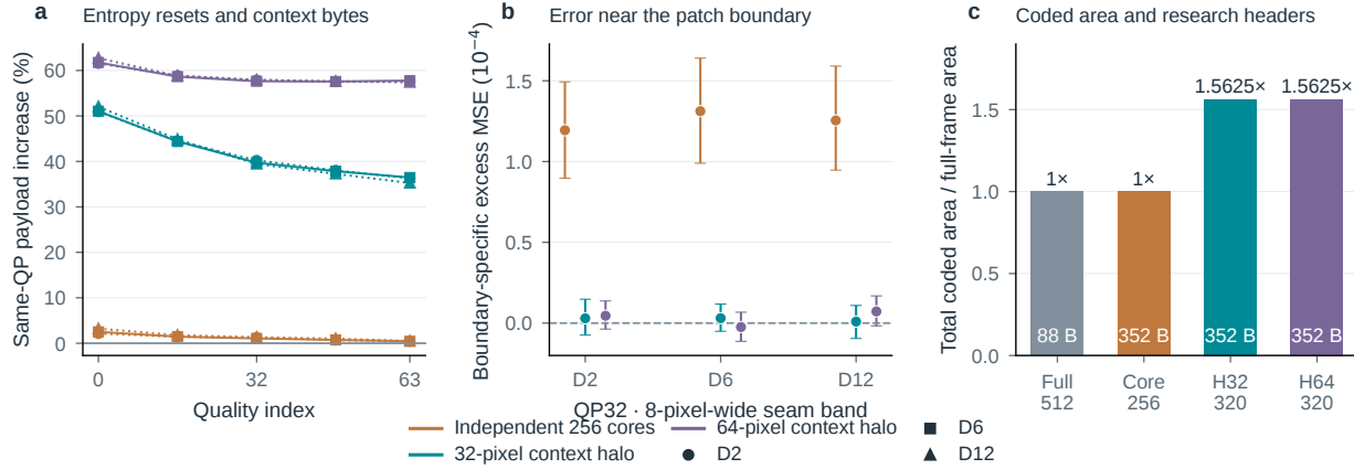
Figure S28. A better seam and a better codec are different outcomes. a , Same-QP payload increase over the full-frame model. b , At QP32, patch-minus-full MSE in the central 8-pixel seam band, minus the corresponding interior excess. c , Exact coded area and research-header bytes. Halo32 and halo64 have equal coded area under this padding policy, but different real context. Area ratios are not latency ratios, and same-QP seam diagnostics are not equal-rate quality comparisons.
