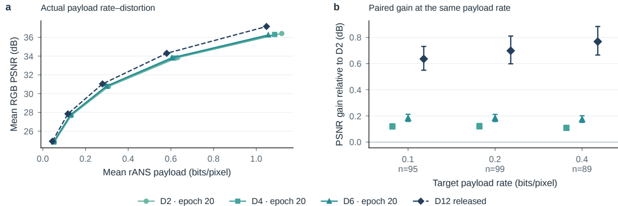
Figure S16. Shallow models are close, but not identical, at equal coded rate. a , Mean RGB PSNR and actual payload over all 100 crops at five QPs; joining lines are visual guides. b , Per-image interpolation and paired differences on four-model common support, with 95% image-bootstrap intervals. D2/D4/D6 are frozen epoch-20 models; released D12 is not matched in training history. These measured streams establish an interim CPU rate–distortion comparison, not final quality or native runtime.
