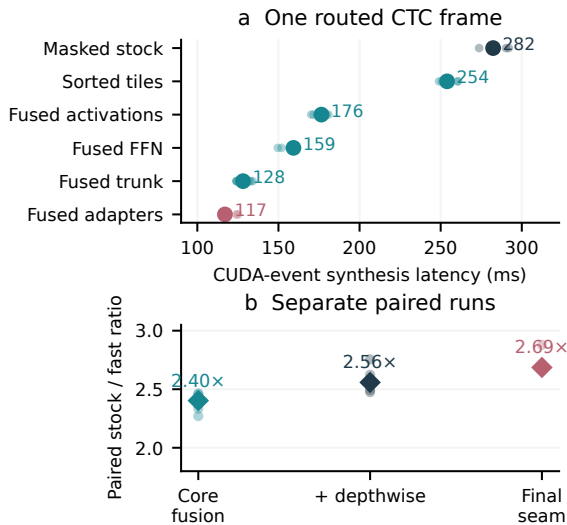
Figure S33. An implementation gain on one real routed frame. a , Six shuffled, paired CUDA-event trials of consecutive kernel stages. Dots are trials and large marks are medians. b , Three separately timed implementations; ratios are paired within each run but cannot be compared as an incremental ablation across runs because GPU contention changed. CTC videoSRC05 at QP32, 1920 \times 1080 valid pixels padded to 2048 \times 1280 , with exit-6/8/10/12 tile counts 13/20/4/3. The GPU was shared with training.
