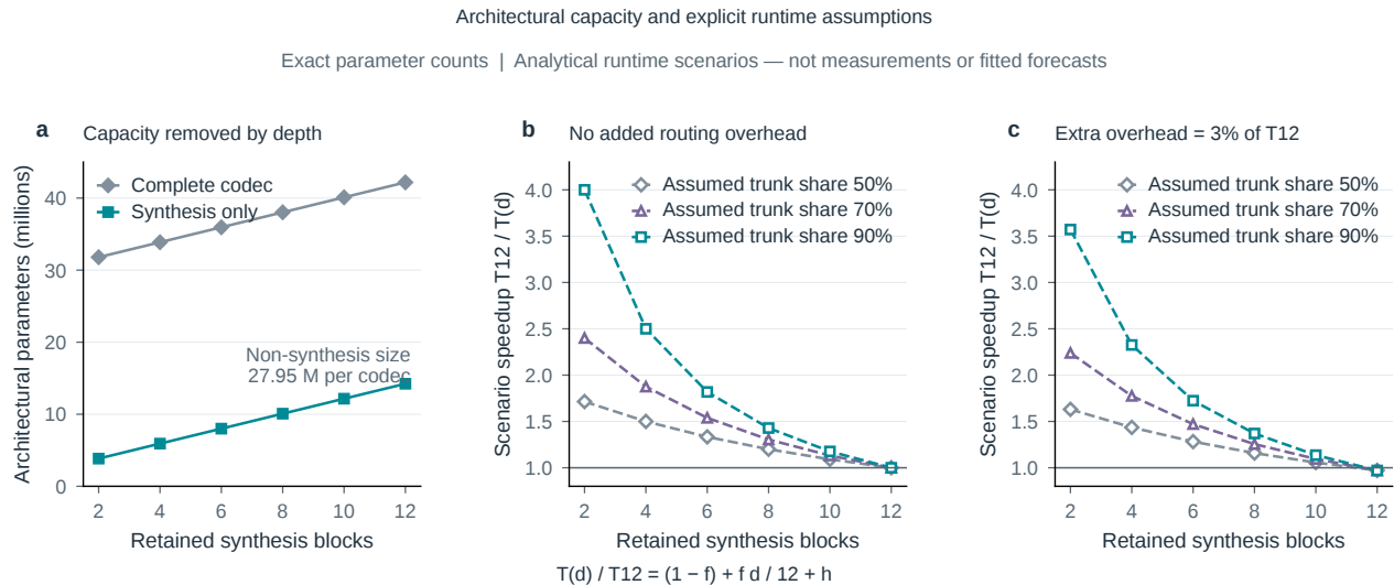
Figure S22. A transparent design-space illustration for unfinished experiments. a , Exact architectural parameter counts. b,c , Analytical runtime sensitivity to assumed trunk-time share and added overhead. Open markers and dashed lines denote assumptions, not measurements or fitted forecasts. No quality or bitrate outcome is assigned to an unfinished model.
