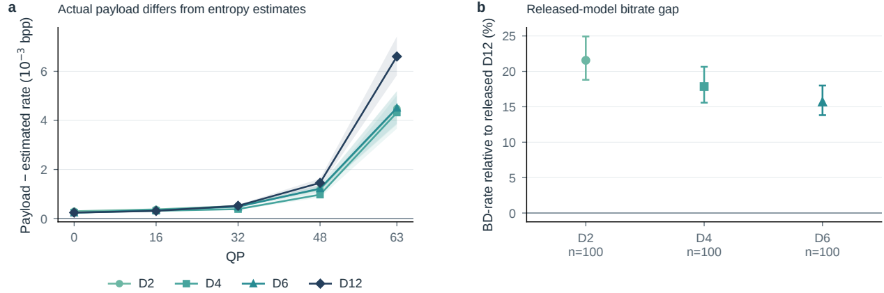
Figure S18. Estimated entropy and emitted bytes are separate quantities. a , Actual rANS payload minus entropy estimate, excluding the research header. b , Mean per-image BD-rate against the released anchor on each image’s four-model common PSNR interval. Intervals resample images; no uncertainty from independent training seeds is represented.
