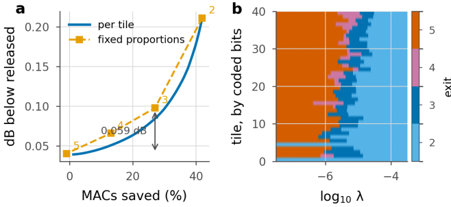
Figure 7. The two achievable sets, on one frame. a , the per-tile frontier of Theorem 4 traced by sweeping \lambda , against the fixed-proportion chain of Proposition 3 through the four uniform-depth points, labelled by exit. The per-tile curve lies below the chain everywhere between the vertices, by 0.059 dB at the exit-3 vertex. b , the exit each of the 40 tiles takes as \lambda rises, tiles ordered by the bits the entropy coder spent on them. Every row is non-increasing, which is Proposition 2 per tile, and the rows differ, which is what Theorem 4 buys over Proposition 3. The bottom row is a tile that never leaves the shallowest exit.
