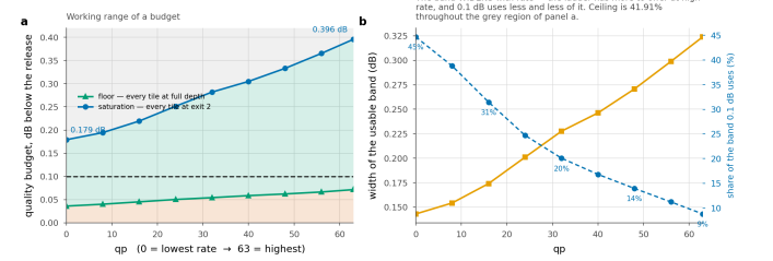
Figure 12. Three regions, and only the middle one is a design choice. Below the floor no allocation meets the budget; above saturation every tile is already on the cheapest rung. The working 0.1 dB budget uses 45% of the window at the lowest rate and 9% at the highest.
