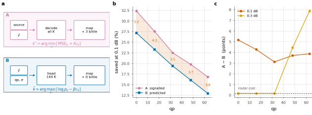
Figure 17. Who decides. (a) The two decision paths of Section 3.1, drawn side by side: the encoder's search over all K exits per tile against the head's forward pass over decoded data. (b) Saving at 0.1 dB; shading is what a bit-exact bitstream costs. (c) That cost is smallest at q32, where the router needs almost no cost multiplier to reach the budget from where it was trained, and grows in both directions. At 0.3 dB it falls to the router's own 0.163% wherever the budget saturates the ladder, and widens where it does not.
