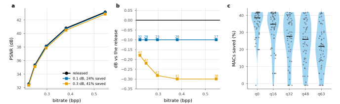
Figure 10. The plane a codec is read on, and the spread behind the mean. a, operating points against the released curve. b, the same with the quality axis expanded; labels are compute saved. c, per sequence at a matched point near 0.1 dB; one dot per sequence, bar is the median.
