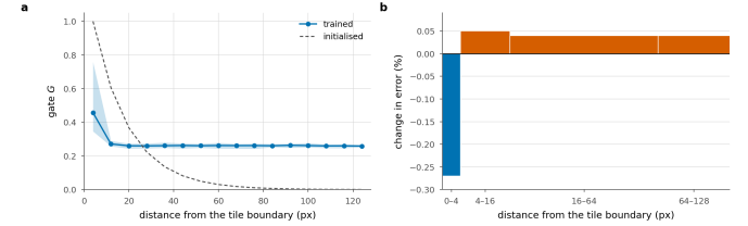
Figure 8. A learned deblocking filter. A correction gated by position within a tile, applied once to the stitched frame, for 0.95% of the decode. a , the gate against distance from the tile boundary, beside the initialisation it started from; shading is the spread over cells at the same distance. The trained gate keeps the ring, up to 0.76 at a tile corner, and then flattens at 0.26 instead of switching off. b , the change in error measured with the filter on, by distance from the nearest tile boundary; bar width is the share of pixels, so bar area is what a ring contributes to the frame. It wins 0.27% on the 6.2% of pixels within 4 px of a boundary and loses 0.04 to 0.05% on the 94% beyond it.
