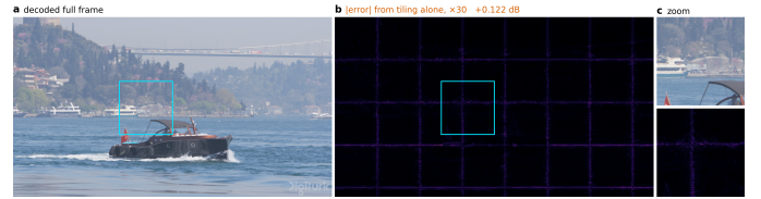
Figure 5. The artefact, before anything is done about it. Bosphorus at 1080p, quality index 63, stock zero padding at the tile border. a , one frame decoded from the bitstream in one piece. b , the same bitstream, the same weights, every tile at full depth and no early exit anywhere, decoded in 256 pixel tiles: the absolute difference between the two decodes, amplified 30 times. The only thing that changed is that the second decode was tiled, and the error it produces is the tile lattice and nothing else. c , the boxed region of each.
