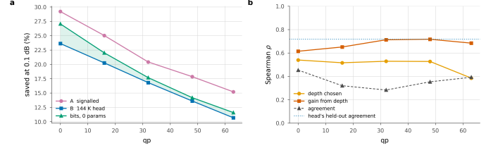
Figure 28. The calibrated bit rule. a, saving at 0.1 dB; shaded where the calibrated bit rule beats the trained head. b, what a tile's bit count is correlated with, against how often the rule agrees with the oracle outright; dotted is the head's own held-out agreement.
