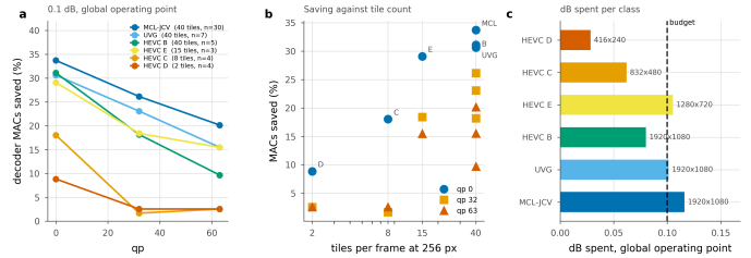
Figure 21. Saving by test class at one global operating point. \lambda is bisected once so the whole set lands on the budget, exactly as it would be in deployment; each class is then reported at that \lambda . The ordering follows tile count, not content.
