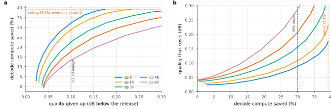
Figure 25. The trade-off, whole. a, what a budget buys, per rate; the dotted line is the arithmetic ceiling, 39.1%, and q0 reaches it at 0.179 dB. b, the same relation inverted, so it reads as what a saving target costs. The three budgets reported elsewhere are three points on this curve.
