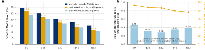
Figure 30. Three ways to choose an exit. a , saving at 0.1 dB. The encoder search sees the source and sends 89 bits a frame; the other two send nothing. The bit rule beats the trained head at every rate, with no learned parameters against the head's 144,030. b , bars are the tiles where the rule picks the search's exit, the line the fraction of its saving it captures anyway.
