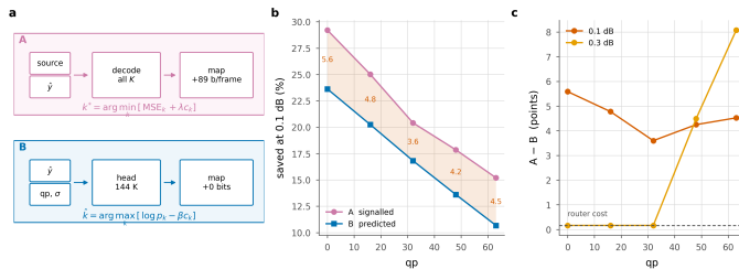
Figure 27. Who decides. a, the two decision paths side by side: the encoder's search over all K exits per tile against the head's forward pass over decoded data. b, saving at 0.1 dB; shading is what a bit-exact bitstream costs. c, that cost is smallest at q32 and grows in both directions.
