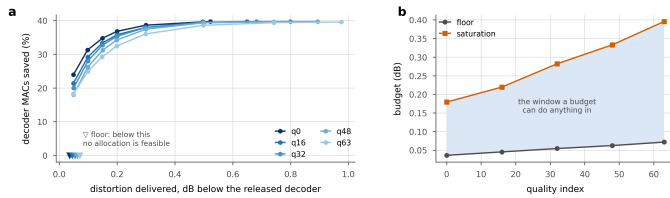
Figure 26. The window a budget works in. a, saving against the distortion actually delivered, per rate. Every curve begins at a floor, below which no allocation meets the budget, and flattens at a saturation point, above which a looser budget buys nothing. b, those two limits against rate. The shaded band is the only region in which a budget is a design choice rather than a formality.
