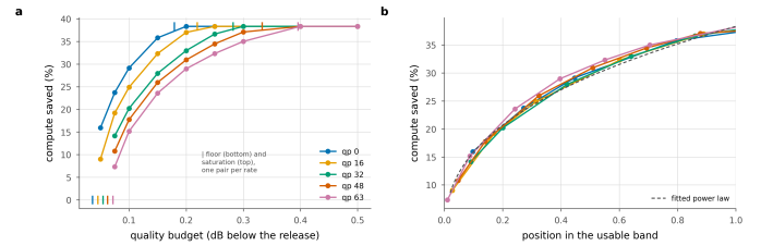
Figure 24. The band is the rate dependence. a , saving against the budget, with each rate's floor and saturation point ticked. b , the same with the budget axis rescaled onto each rate's own band. Five curves become one; dashed is the one-parameter power law fitted to all of them.
