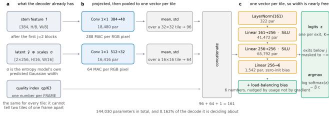
Figure 58. The router head. a , the three things it reads, all already held by the decoder at the moment the decision is needed. b , each projected by a 1 \times 1 , then reduced to one vector per tile by its mean and standard deviation. c , a three-layer perceptron, one pass per tile. Every shape and parameter count in the figure is read off the module when the figure is drawn.
