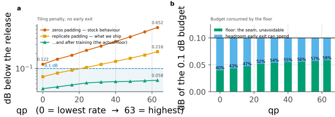
Figure 53. The tiling penalty across the whole rate range, every tile at full depth, so this is the floor and nothing else. a, the steps that reduce it, of which the two that matter cost no arithmetic; the largest single factor is training the ladder with the seam present. b, the floor as a share of the 0.1 dB budget: it is charged inside the budget and consumes a growing part of it as the rate rises, which is one of the two reasons the saving falls with rate.
