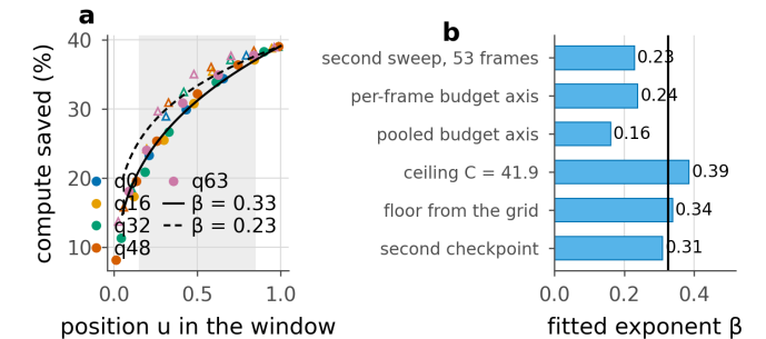
Figure 56. The collapse, and what the exponent is sensitive to. a , the rescaled points from two sweeps of the pinned checkpoint, filled circles for the 106-frame grid and open triangles for the 53-frame frontier, with the power law fitted to each over the shaded window. The two sweeps of one checkpoint do not lie on one curve. b , the exponent under one change at a time, with the vertical line at the exponent of the first row of Table 75. The change of checkpoint, which the main paper reads as a finding, is the smallest of the six.
