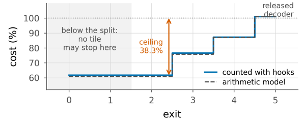
Figure 39. The ladder, priced. What a tile costs at each exit, as a percentage of one released decode, counted with hooks on the executed pass and beside the arithmetic model the argmin uses. Exits below the split depth are not distinct, because the first j groups run for every tile whatever it does. The deepest exit costs slightly more than the release, which is the full-frame deblocking pass. Reported savings in the paper are the hook count.
