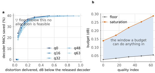
Figure 52. The window a budget works in. a, saving against the distortion actually delivered, per rate. Every curve begins at a floor, below which no allocation meets the budget, and flattens at a saturation point, above which a looser budget buys nothing. b, those two limits against rate. The shaded band is the only region in which a budget is a design choice rather than a formality. The main paper states both limits; this is them drawn.
