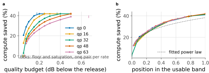
Figure 54. The collapse on the second training run. a , saving against budget, one line per rate, with each rate's floor and saturation point ticked. b , the same with the budget axis rescaled onto each rate's own window; dashed is the one-parameter power law. The main paper shows this pair for the pinned checkpoint.
