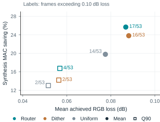
Figure 8. Fixed controls trade saving against quality risk. Actual reconstructions on all 53 QP32 frames. Colour identifies the policy; filled circles and open squares denote mean and Q90 calibration. Labels count RGB losses above 0.1 dB. Axes report achieved RGB loss against e15 full-frame and modelled synthesis MAC saving. Controls fitted on other sequence folds do not match achieved quality.
