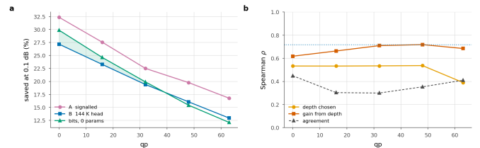
Figure 25. The calibrated bit rule. a Saving at 0.1 dB; shaded where the calibrated bit rule beats the trained head. b What a tile's bit count is correlated with, against how often the rule agrees with the oracle outright; dotted is the head's own held-out agreement.
