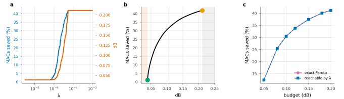
Figure 20. The structure of the allocation , on one frame. a , compute and distortion are monotone in the multiplier. b , the frontier between floor and saturation; shaded regions are infeasible or wasted. c , what the Lagrangian reaches against the exact Pareto set, enumerated by dynamic programming.
