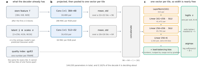
Figure 9. The router head. a , the three things it reads, all already held by the decoder. b , each projected by a 1 \times 1 , then reduced to one vector per tile by its mean and standard deviation. c , a three-layer perceptron, one pass per tile. Every shape and parameter count is read off the module when the figure is drawn.
