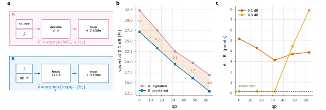
Figure 24. Who decides. a , the two decision paths side by side: the encoder's search over all K exits per tile against the head's forward pass over decoded data. b , saving at 0.1 dB; shading is what a bit-exact bitstream costs. c , that cost is smallest at q_{32} and grows in both directions.
