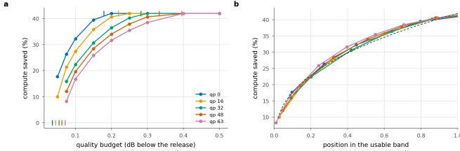
Figure 21. The band is the rate dependence. a Saving against the budget, with each rate's floor and saturation point ticked. b The same with the budget axis rescaled onto each rate's own band. Five curves become one; dashed is the one-parameter power law fitted to all of them.
