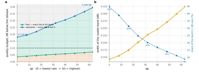
Figure 19. Three regions, and only the middle one is a design choice. Below the floor no allocation meets the budget; above saturation every tile already takes the cheapest exit. The 0.1 dB budget uses 45% of the band at the lowest rate and 9% at the highest.
