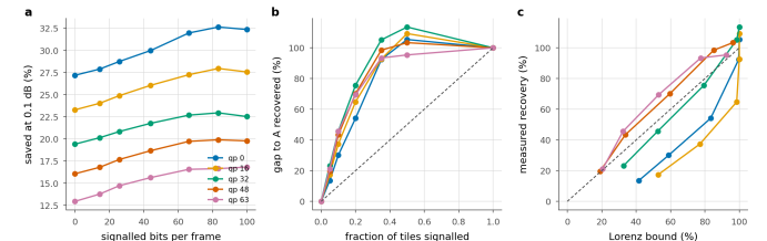
Figure 27. Partial signalling. a, saving against the bits spent on the map; each line runs from B on the left to A on the right. b, the same normalised by the A-to-B gap; dashed is proportional recovery. c, against the fixed- \lambda Lorenz bound; points above the dashed line are allocations one multiplier cannot reach.
