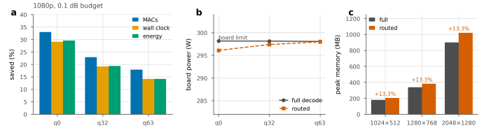
Figure 30. Three units for one saving. a , the same routed decode measured as arithmetic, as wall clock and as joules per frame, at 1080p and a 0.1 dB budget. Energy follows the clock, not the arithmetic. b , why: the board draws the same power either way, because the later groups run on a shrinking set of tiles and a partly idle GPU still draws its static power. c , peak memory, which routing raises rather than lowers, by 13.3% at every resolution that fitted on the card.
