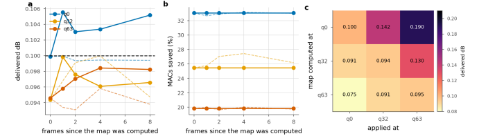
Figure 29. Reusing an exit map. Solid is the transferred map, dashed the one recomputed in place. a , b : reuse across frames of the same sequence. c : reuse across quality index; the entry is the delivered distortion against a 0.1 dB budget.
