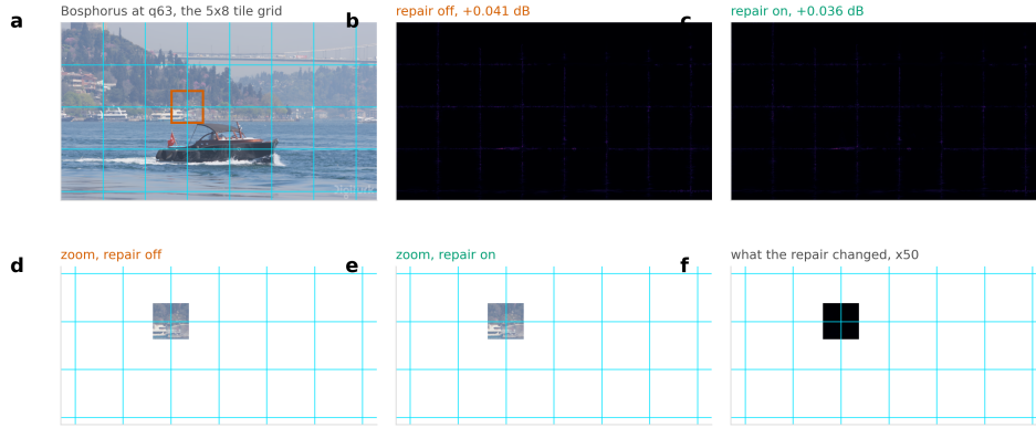
Figure 15. What the deblocking pass does to a picture. Bosphorus at q63, the rate where the seam is worst, decoded twice from one latent with every tile at full depth. a , the frame and its 5×8 grid. b , c , the error against a full-frame decode of the same latent, amplified 25 times, with the pass off and on. d , e , one grid crossing in the picture itself. f , what the pass changed there. It recovers 0.005 dB of the 0.041 dB that tiling costs on this frame, which is the measurement behind the section title.
