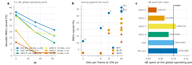
Figure 18. Saving by test class at one global operating point. \lambda is bisected once so the whole set lands on the budget, exactly as it would be in deployment; each class is then reported at that \lambda . The ordering follows tile count, not content.
