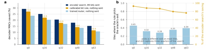
Figure 26. Three ways to choose an exit. a, saving at the 0.1 dB budget. The encoder search sees the source and sends 89 bits a frame; the other two send nothing. The bit rule beats the trained head at every rate, by the margin printed above it, with no learned parameters against the head's 144,030. b, bars are the tiles on which the rule picks the exit the search would have, and the line is the fraction of the search's saving it nonetheless captures. Picking a different exit on most tiles costs it far less than picking a different exit sounds like it should, which is the case against training a router on exit labels.
