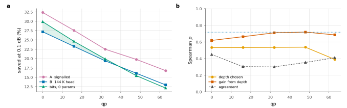
Figure 25. The calibrated bit rule. a Saving at 0.1 dB; shaded where the calibrated bit rule beats the trained head. b What a tile's bit count is correlated with, against how often the rule agrees with the oracle outright; dotted is the head's own held-out agreement.
