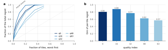
Figure 28. The loss is concentrated. a, the share of the total regret carried by the worst fraction of tiles, per rate; the dotted line is what an even spread would look like. b, the same as a Gini coefficient. At every rate a small minority of tiles carries most of what staying silent costs, which is why signalling a fraction of the map recovers most of the gap.
