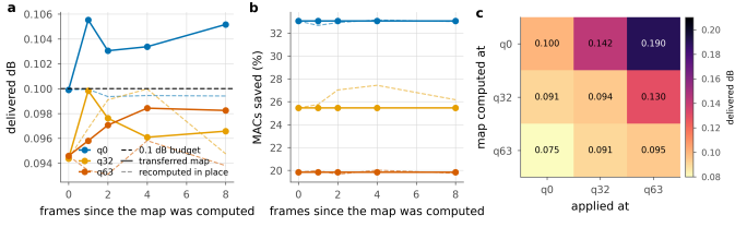
Figure 34. Reusing an exit map. Solid is the transferred map, dashed the one recomputed in place. a, b: reuse across frames of the same sequence. c: reuse across quality index; the entry is the delivered distortion against a 0.1 dB budget.
