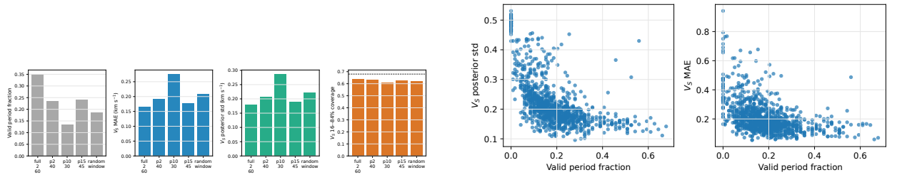
Figure 5. Effect of missing period bands on weak-prior DNN posterior inversion. Left: fixed and random period-window diagnostics for posterior-median V_S error, posterior spread and coverage. Right: random-window relationships between valid period fraction, posterior spread and error.
