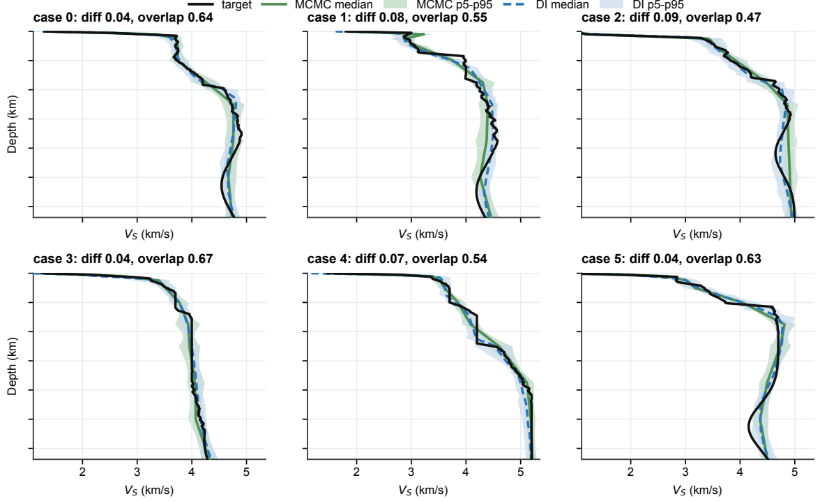
Figure A1. Reduced same-prior MCMC posterior anchor for six inside-support synthetic cases. The MCMC reference uses a 10-knot V_S parameterisation and a Gaussian-mixture prior fitted to projections from the DI-Strong synthetic prior. Lines show posterior medians and shaded bands show pointwise p05–p95 intervals. Inside the synthetic support, DI-Strong gives similar median profiles and comparable interval widths to this reduced Bayesian reference.
