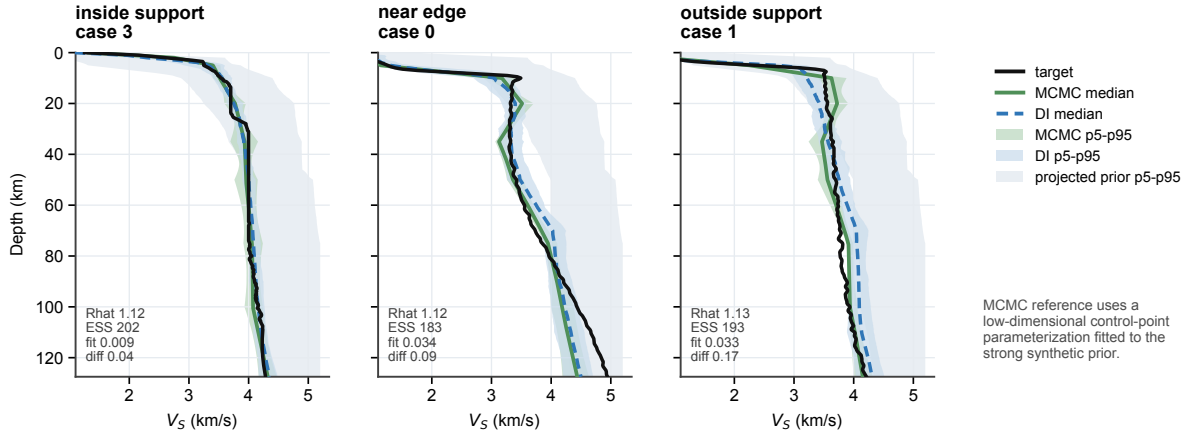
Figure A2. Reduced same-prior MCMC anchor across prior-support regimes. The inside-support case shows close DI–MCMC agreement. The near-edge and outside-support cases show larger differences between the learned posterior and the reduced MCMC reference, even when the posterior-predictive fit remains acceptable. This is why the posterior is interpreted together with prior-support, coverage and posterior-predictive diagnostics rather than as an unchecked Bayesian probability.
