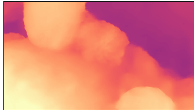
Direct transfer
