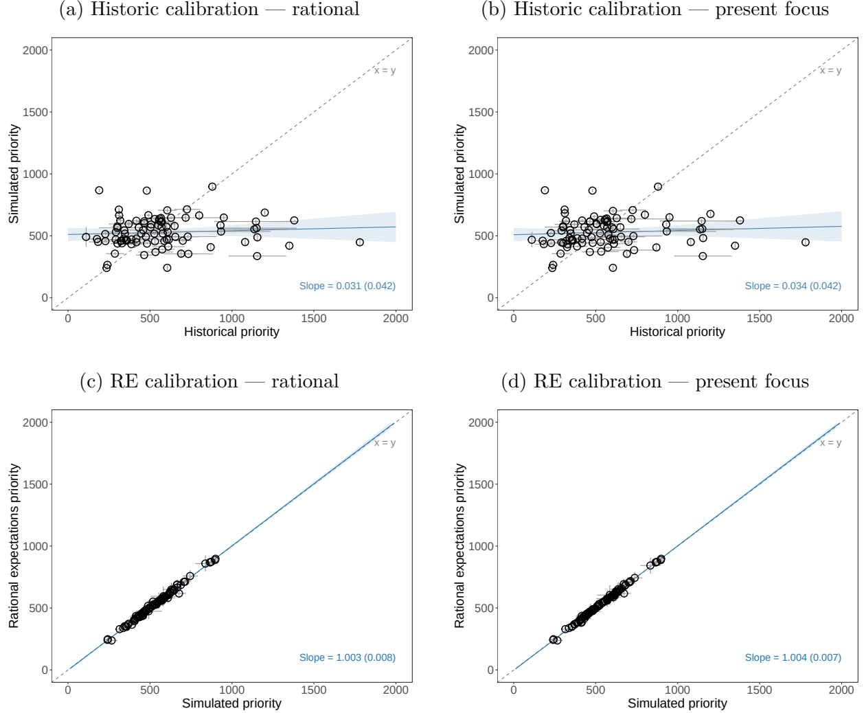
Appendix Figure 15: Simulation validation under US-2
