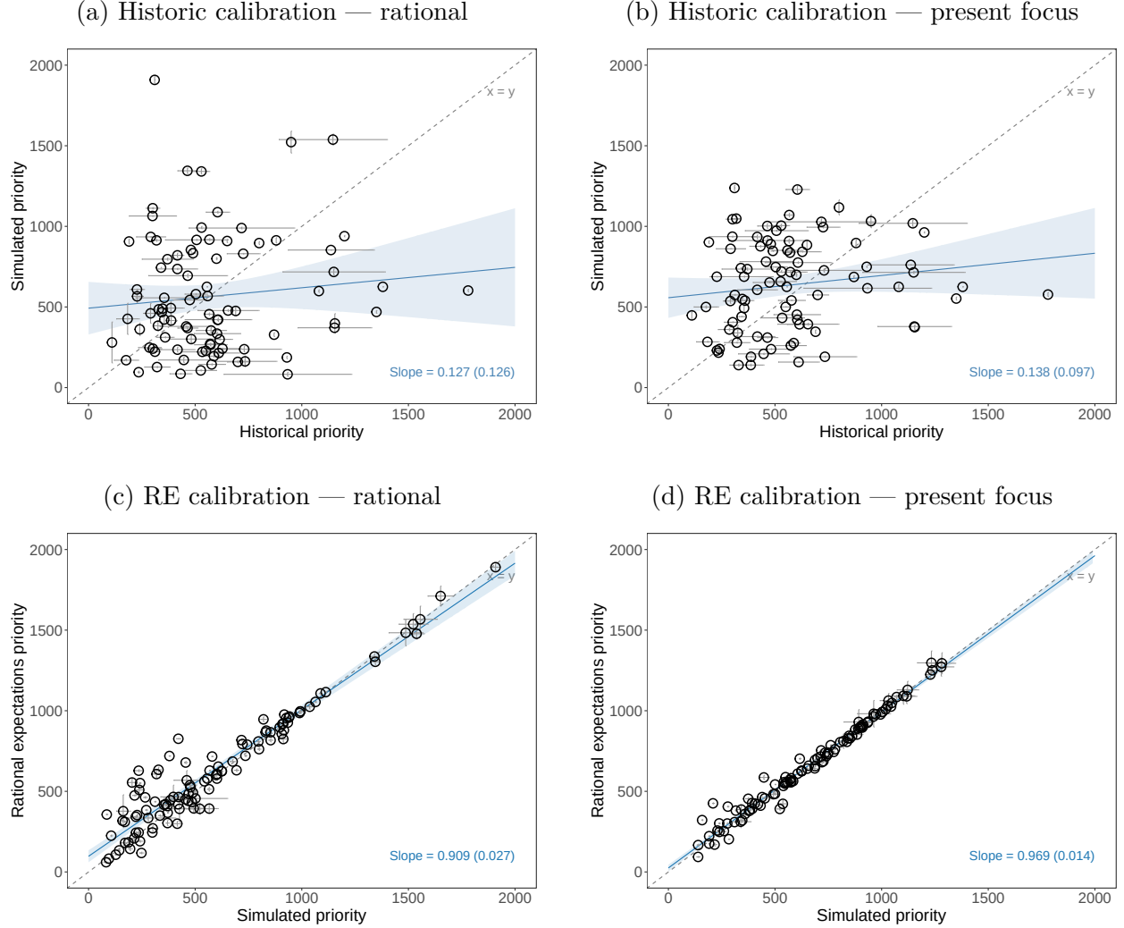
Appendix Figure 14: Simulation validation under UK-3
