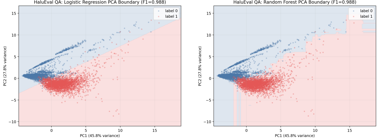
Figure 1: HaluEval QA PCA decision-boundary visualizations with a linear boundary and a Random Forest boundary. The Random Forest plot is more flexible, but both views show strong class separability.
