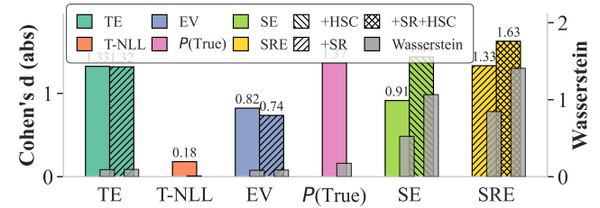
(b) Cohen's d and Wasserstein distance comparisons across methods.
