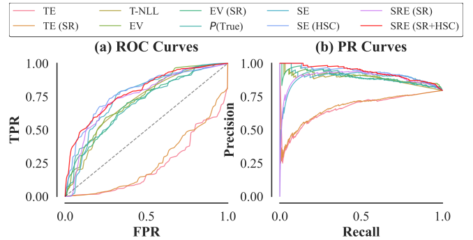
Fig. 3: ROC (a) and PR (b) curves of all methods on SQuAD (no context) with Llama3-8B; for PR, precision is computed on non-hallucinated samples.
