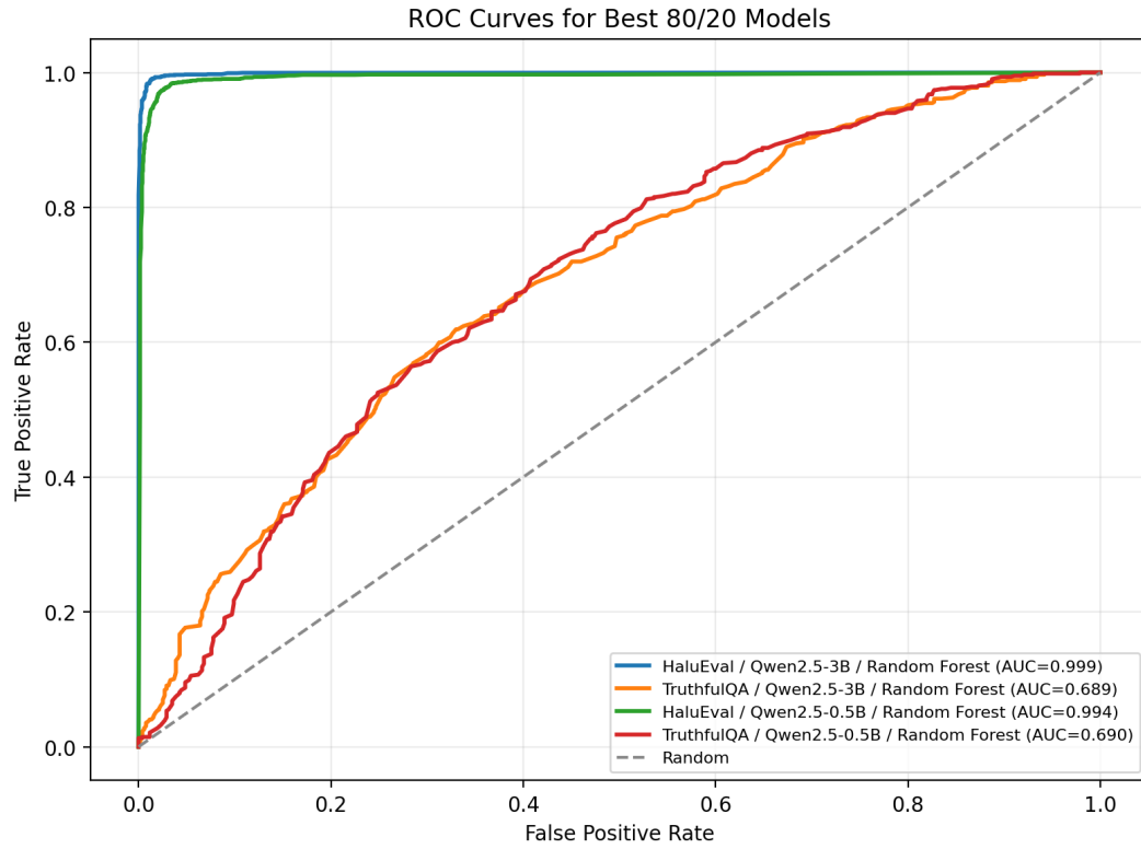
Figure 2: ROC curves for the best grouped 80/20 models.
