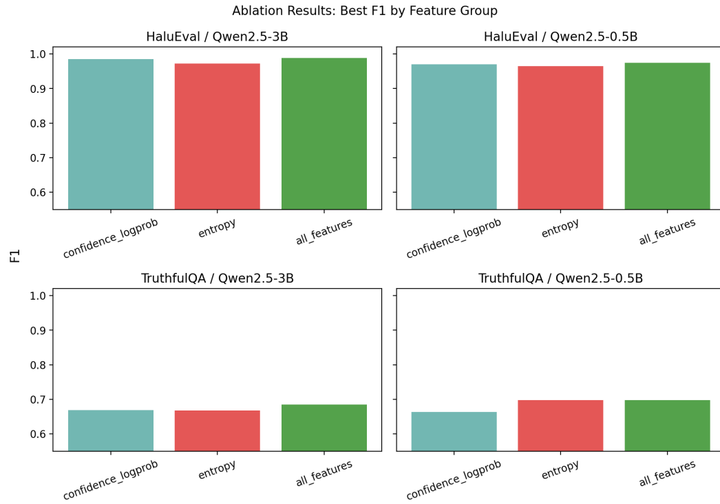
Figure 3: Ablation comparison across confidence/log-probability, entropy, and all feature groups.
